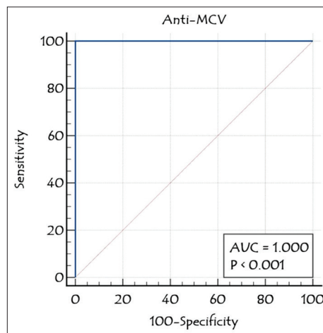
Figure 2: Receiver operating characteristic analysis of anti-mutated citrullinated vimentin in rheumatoid arthritis cases. Anti-MCV: Anti-mutated citrullinated vimentin, AUC: Area under the curve.
