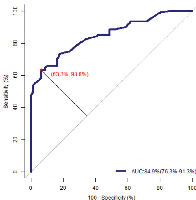
Fig. 1 Receiver operator characteristics curve of test X1 for diagnosing disease A.
